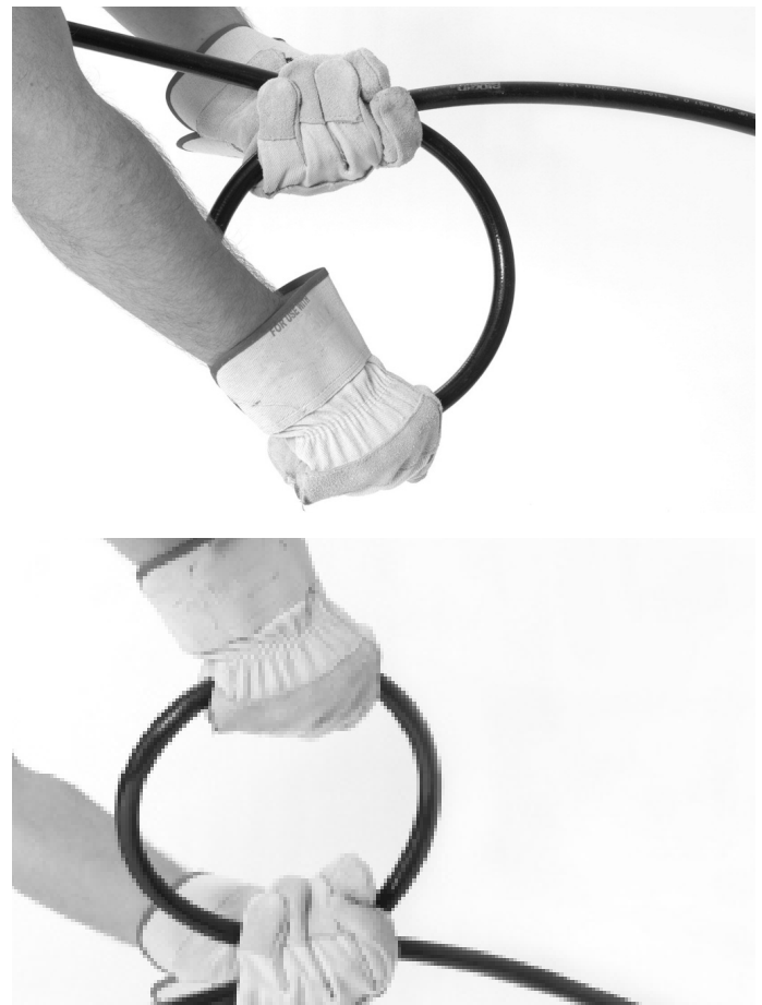
Figure.13 - Hose Operation
