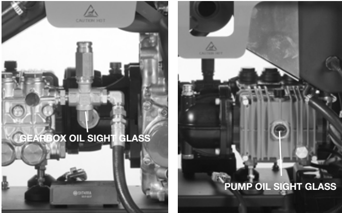
Figure.16 - Checking Pump and Gearbox Oil Level
