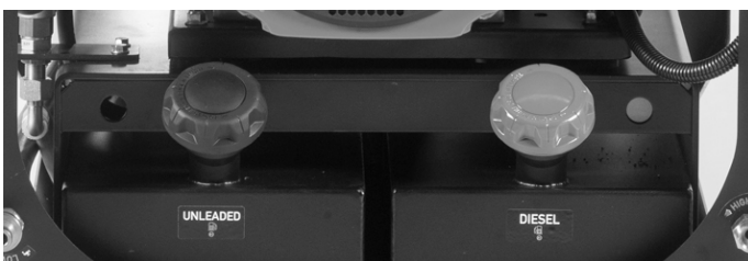
Figure.5A - Diesel fired burner fuel supply tank & Petrol engine fuel supply tank
