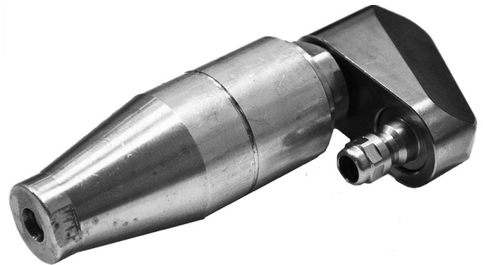
Figure.10 - Reverse Root Cutting Nozzle and Extension Pictured Below
