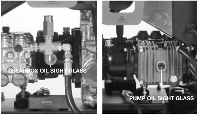
Figure.16 - Checking Pump and Gearbox Oil Level
