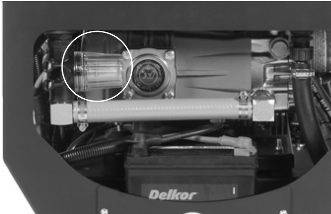
Figure.5 - Scorpion G2 Water Filter
