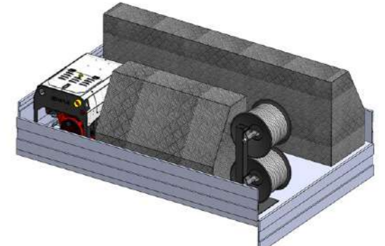
4.1 Ute - Setup 1
