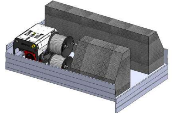
4.2 Ute - Setup 2
