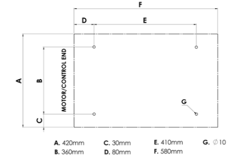
HORNET G2 JNR SKID MOUNTING DATA
