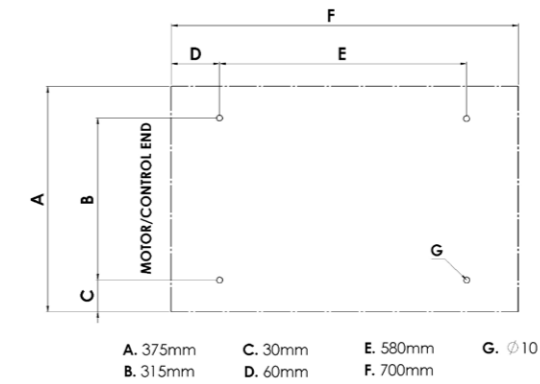
HORNET G2 SKID MOUNTING DATA
