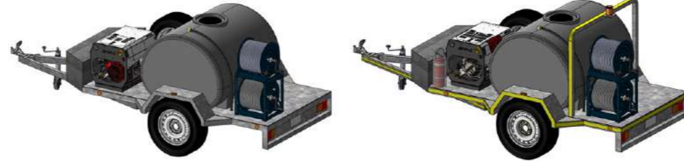
3.1 Trailers - Single Axle 1000L (Hornet G2D Shown with Mine Spec Upgrade)
