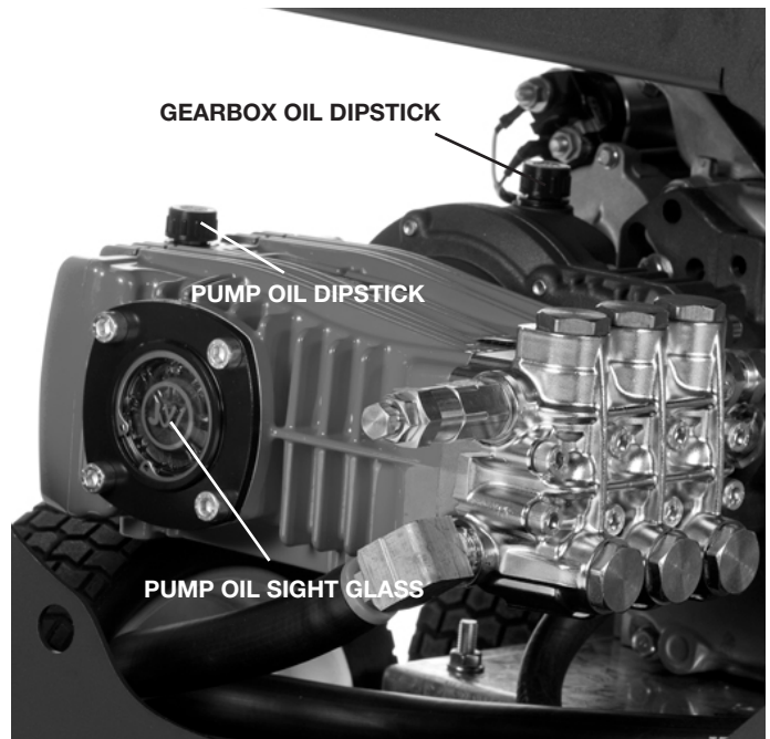
Figure.16 - Checking Pump and Gearbox Oil Level
